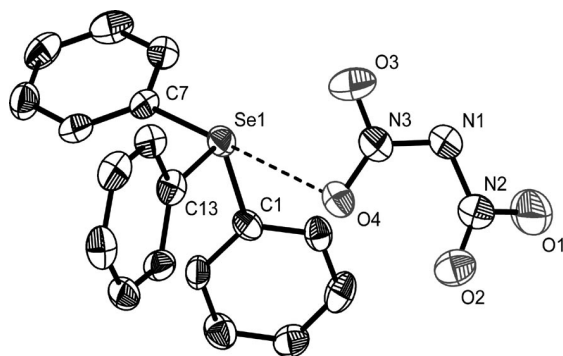
Figure 3. ORTEP plot of the molecular structure of 3 ; H atoms omitted for clarity; selected bond lengths [Å] and angles [°]: Se1–C1 1.927(4), Se1–C7 1.930(4), Se1–C13 1.919(4), Se1...O4 2.979(4), C1–Se1–C7 98.02(16), C1–Se1–C13 103.41(16), C7–Se1–C13 101.03(16).
