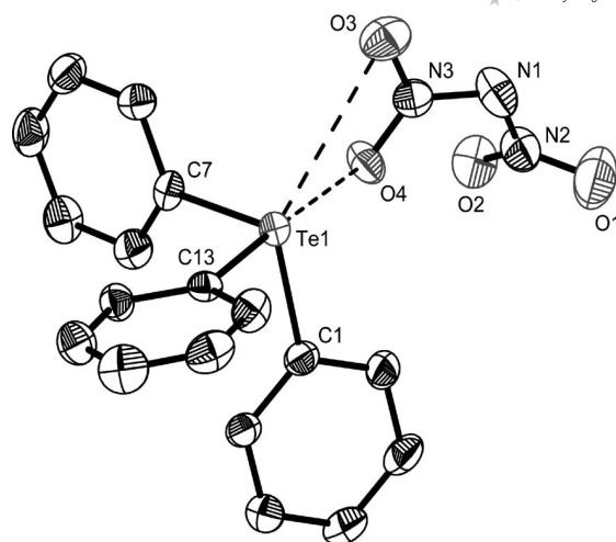
Figure 1. ORTEP plot of the molecular structure of 1 ; H atoms omitted for clarity; selected bond lengths [Å] and angles [°]: Te1–C1 2.112(4), Te1–C7 2.121(4), Te1–C13 2.112(4), Te1 \cdots O3 3.493(3), Te1 \cdots O4 2.952(6), C1–Te1–C7 98.83(14), C1–Te1–C13 93.59(15), C7–Te1–C13 97.67(14), O3 \cdots Te1 \cdots O4 38.03(7).
