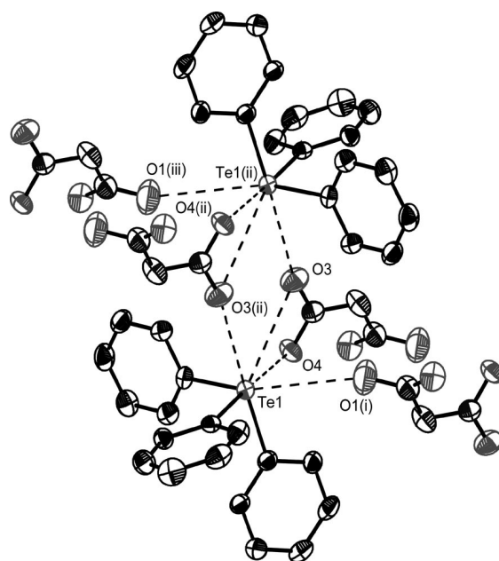
Figure 2. Crystal structure of 1 showing all intermolecular contacts (dashed lines) of the tellurium atoms; H atoms omitted for clarity; selected distances [Å]: Te1 \cdots O1(i)/Te1(ii) \cdots O1(iii) 3.414(1), Te1 \cdots O3(ii)/Te1(ii) \cdots O3 3.089(9), with i = 1 – x, –y, 1 – z; ii = –x, –y, 1 – z; iii = –1 + x, y, z.
